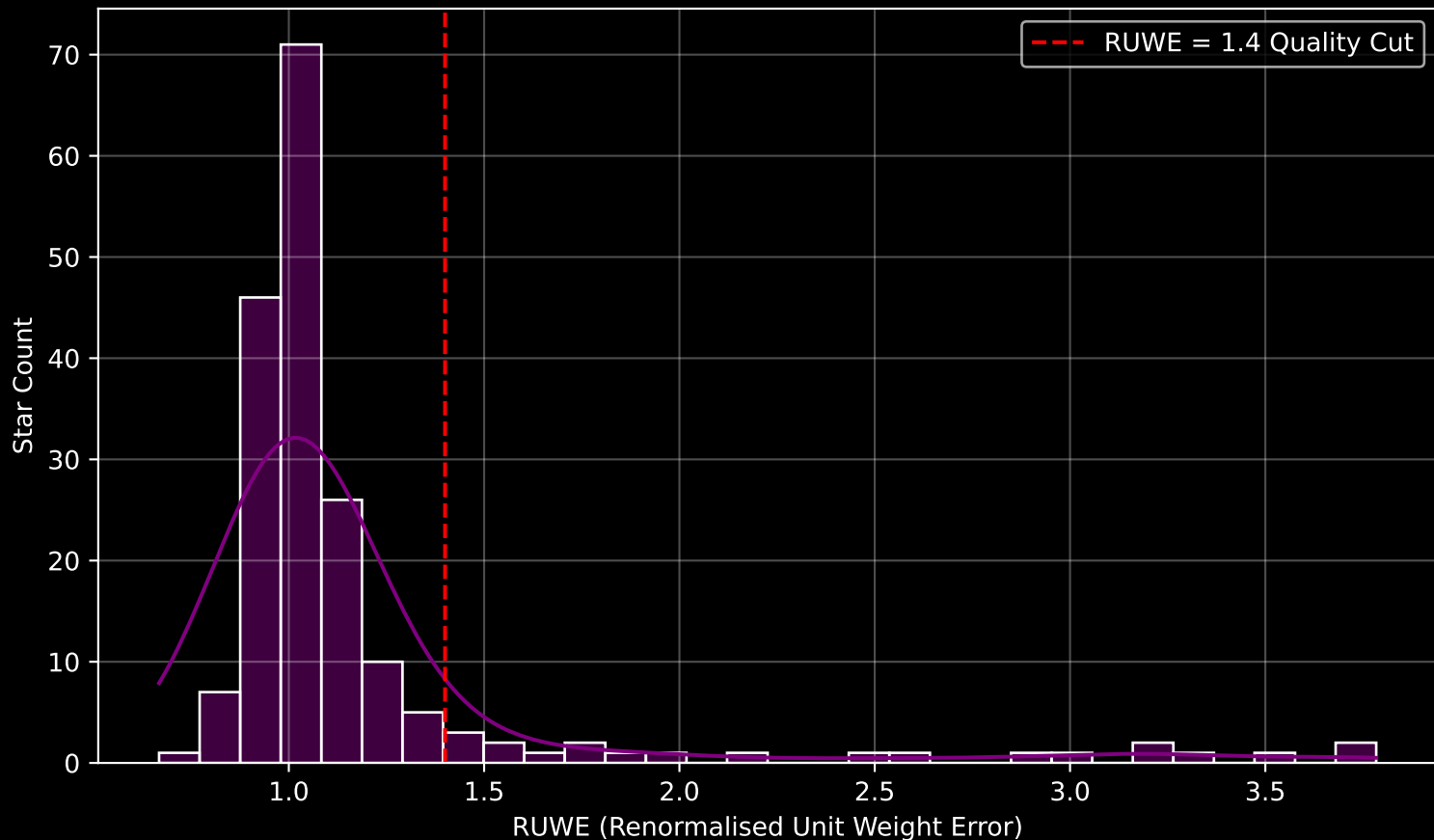
GAPOGEE DR17 Field [193+29_MGA] RUWE Distribution (n= 187)
