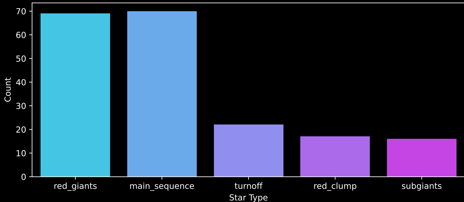
APOGEE DR17 Field: [193+29_MGA] Count plot of Star Type
