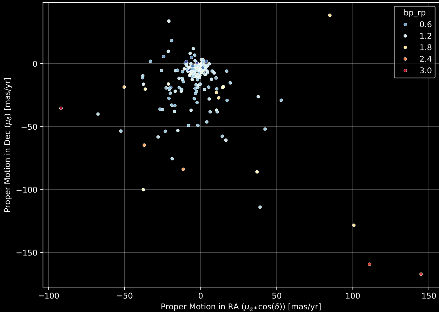
APOGEE DR17 Field: [193+29_MGA] Proper Motion Diagram (n= 194)
