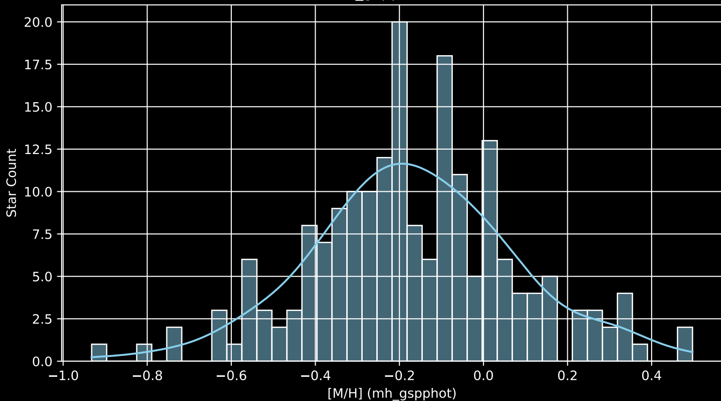
APOGEE DR17 Field: [193+29_MGA [M/H] (mh_gspphot) (n= 193)
