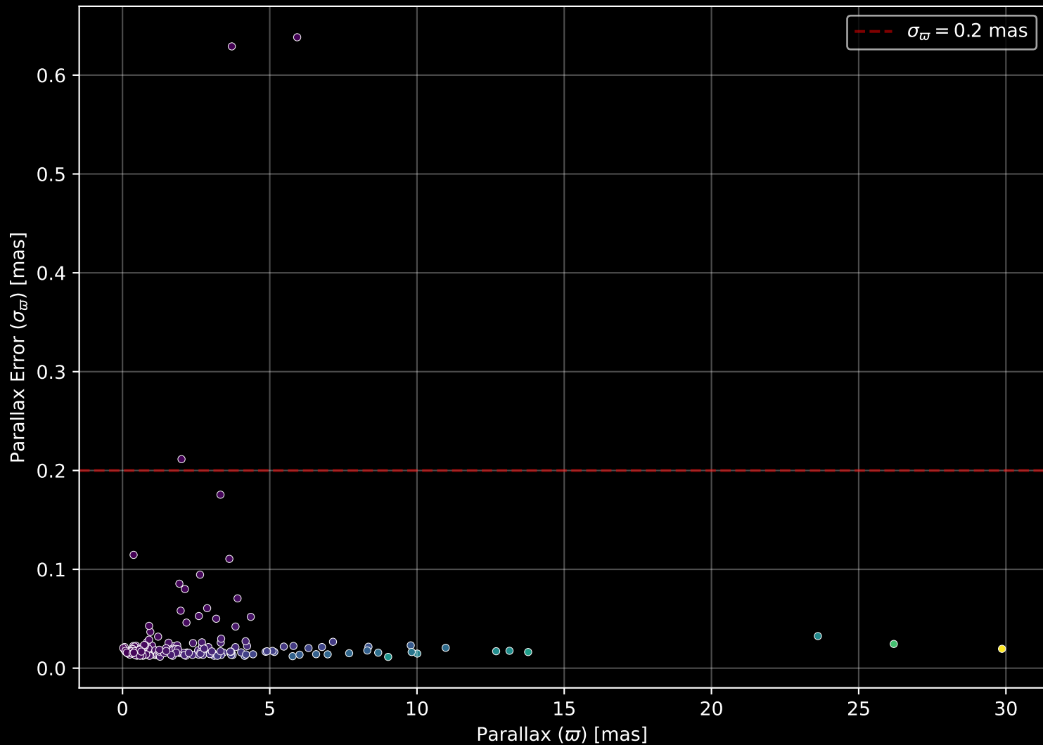
APOGEE DR17 Field: [193+29_MGA] Parallax Quality (n= 194)
