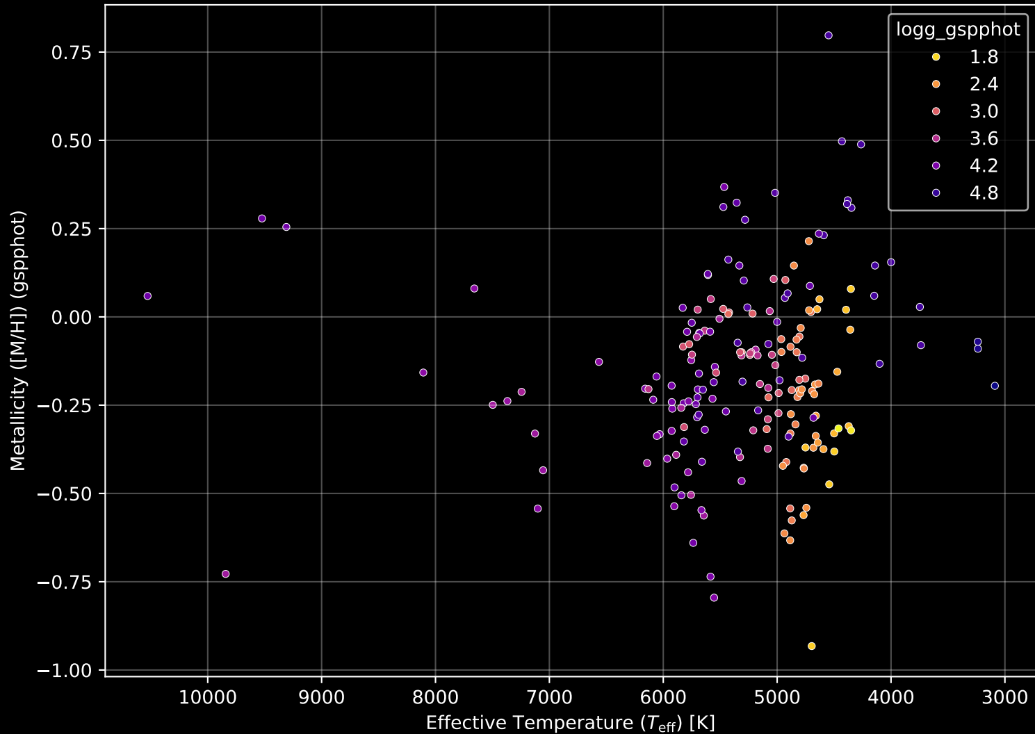
APOGEE DR17 Field: [193+29_MGA] Stellar Population Parameters (n= 194)
